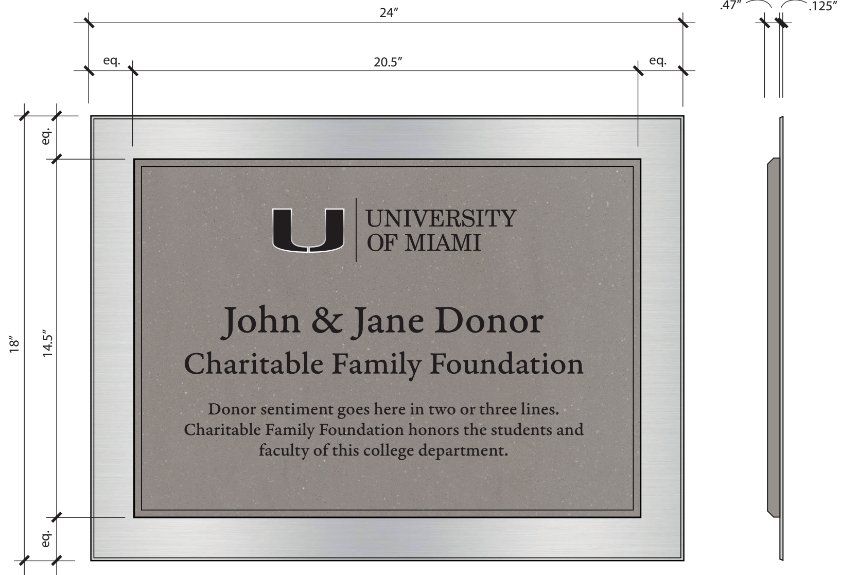
FRONT VIEW
