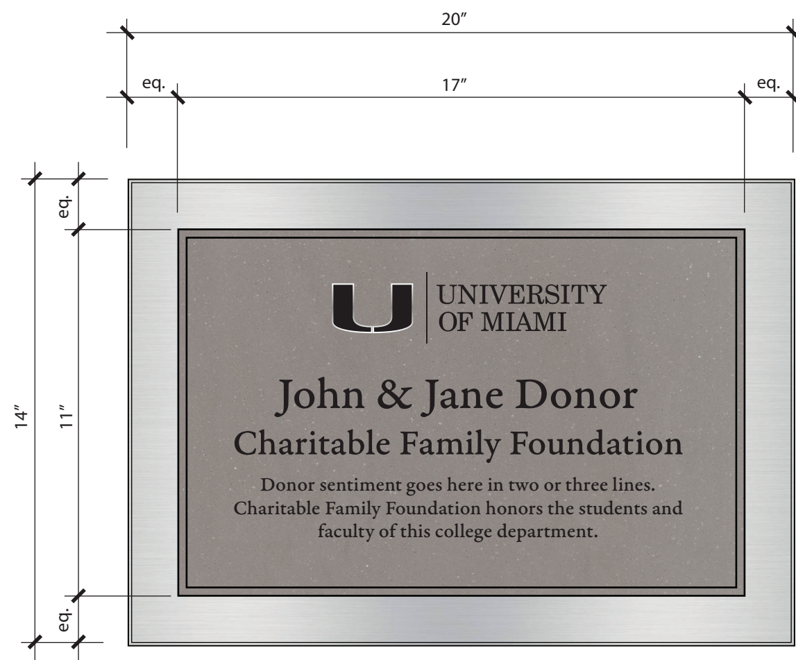
FRONT VIEW
