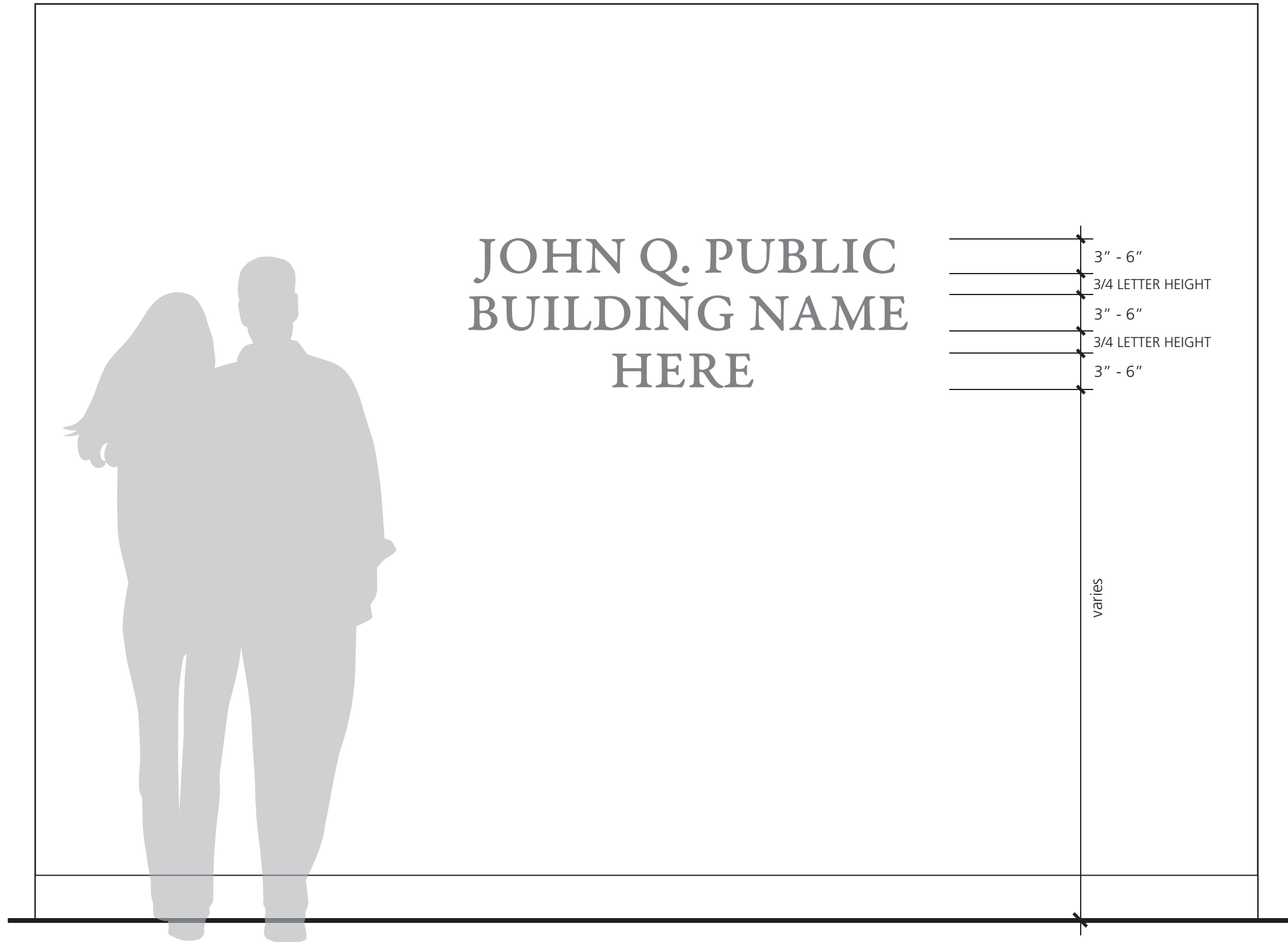
Sign Type UMD-2.0 | Standard Interior Building Identity Sign | General Characteristics - Three Lines of Text
