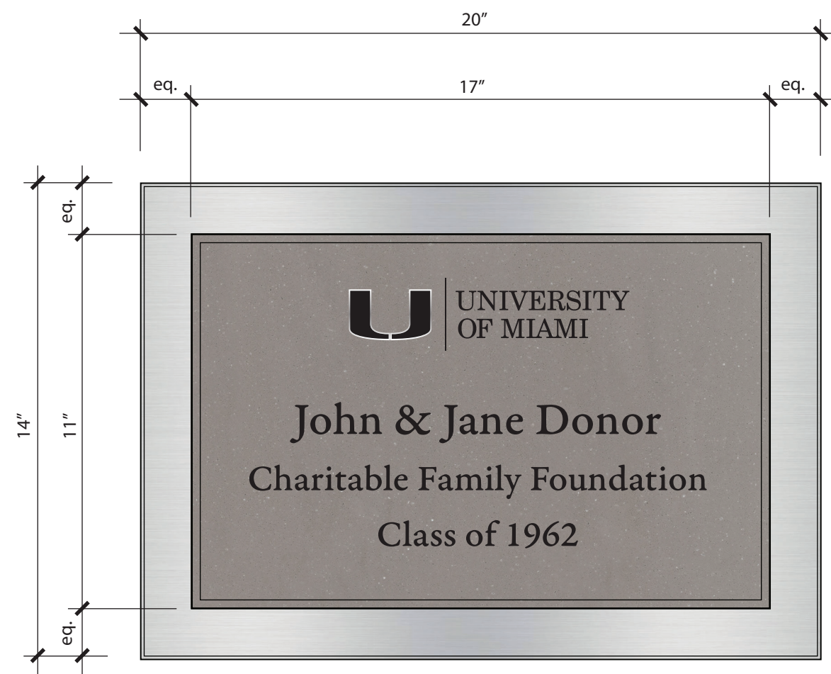
FRONT VIEW
