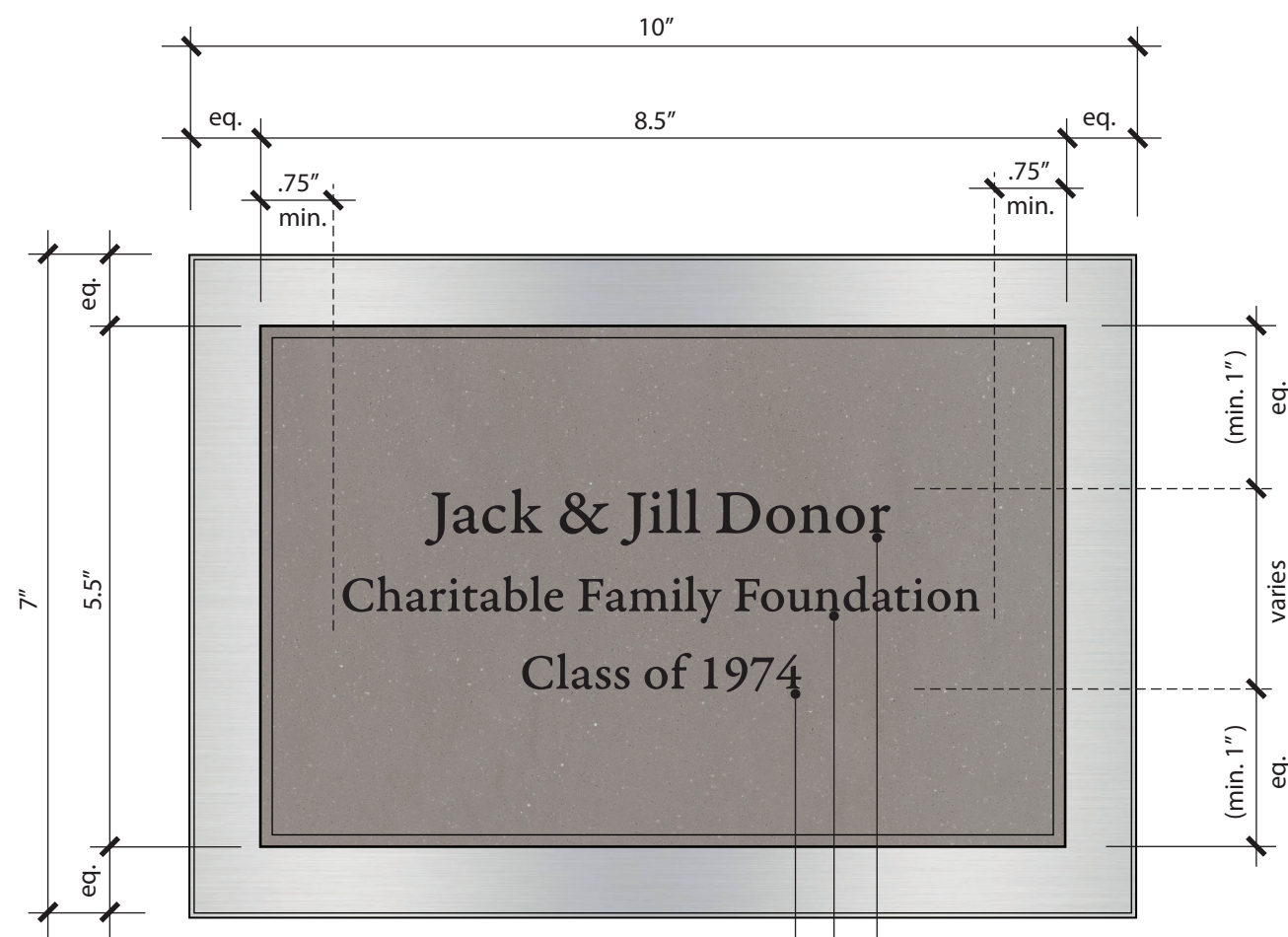
FRONT VIEW
