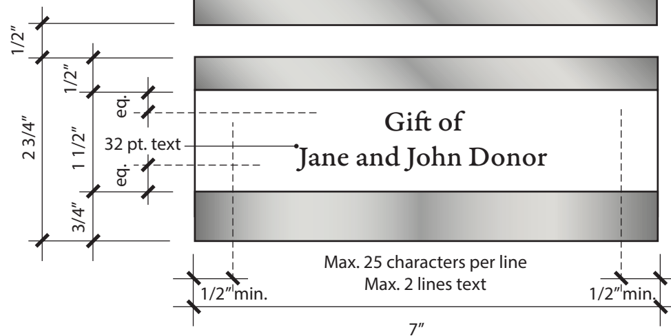
Sign Type: UMD-4.0
