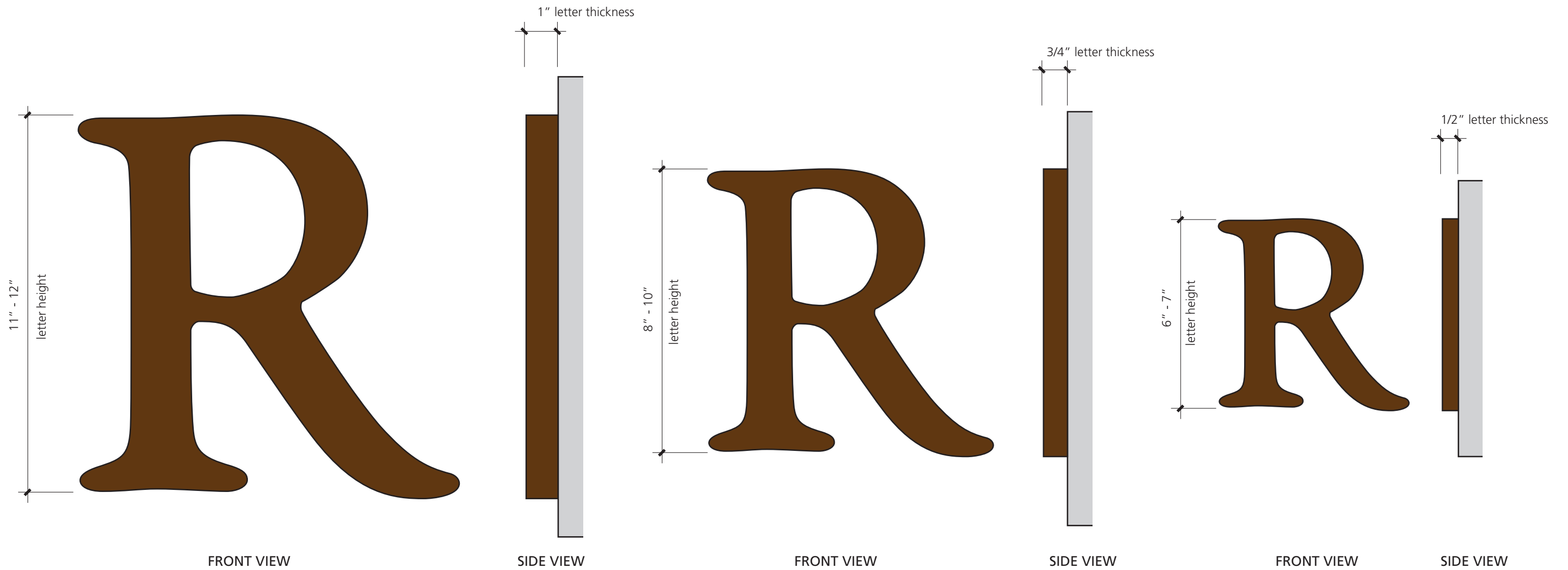
FRONT VIEW
