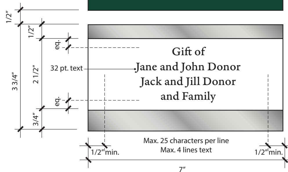
Sign Type: UMD-4.1
