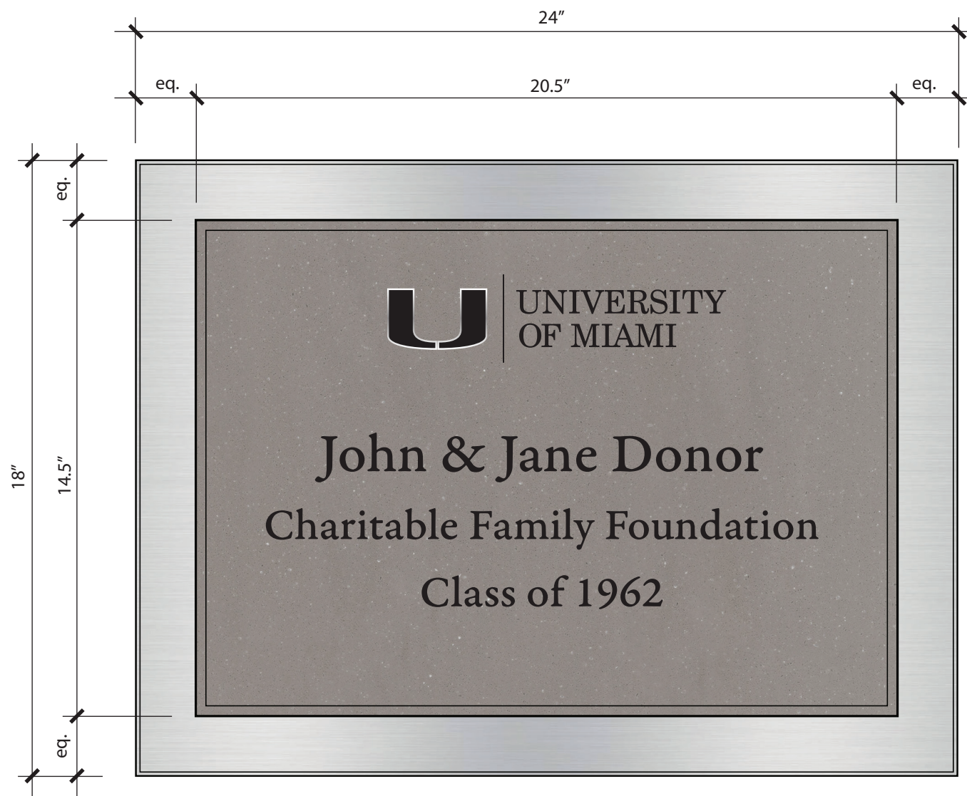
FRONT VIEW
