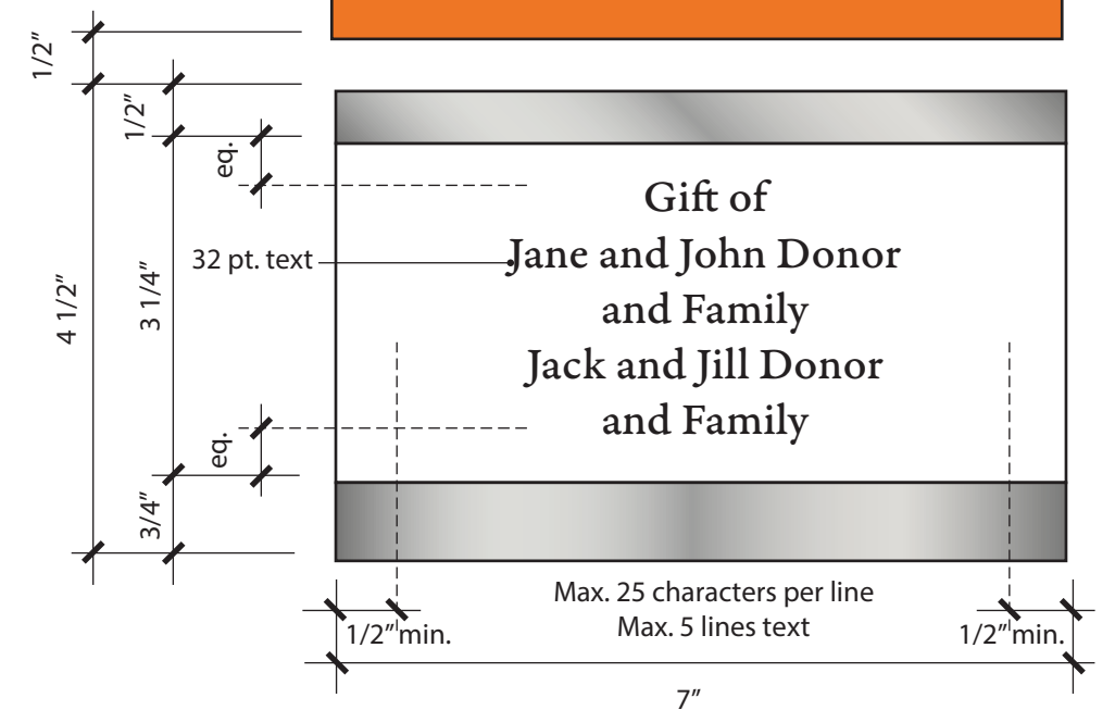
Sign Type: UMD-4.2
